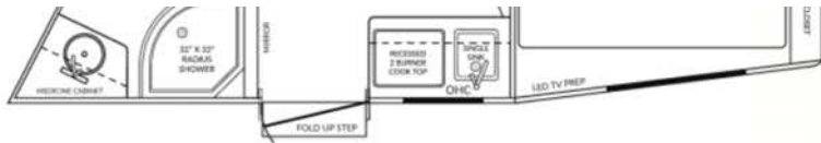
8'8" LIVING QUARTERS - FLOOR PLAN
