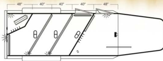
3 HORSE MUSTANG 7' W x 18' L (Floor) x 7' H
