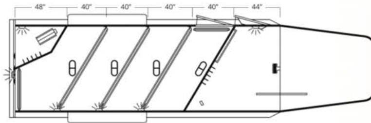
4 HORSE MUSTANG 7' W x 21' L (Floor) x 7' H
