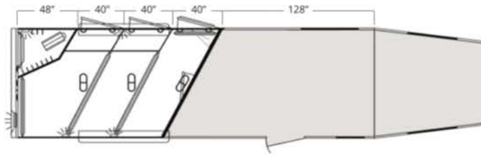
3 HORSE MUSTANG LQ - 10'8" LIVING QUARTERS 8' W x 24'8" L x 7'6" H
